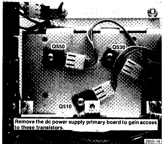
Fig. 5-11. NPN series pass transistors.
