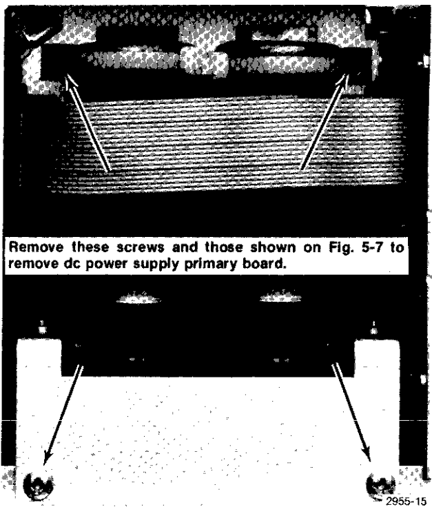
Fig. 5-8. Partial dc power supply primary board removal.
