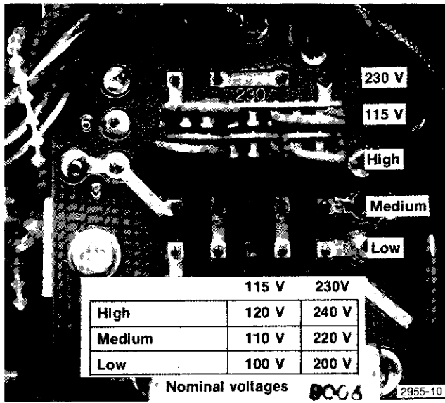
Fig. 5-2. Line voltage jumper positions.
