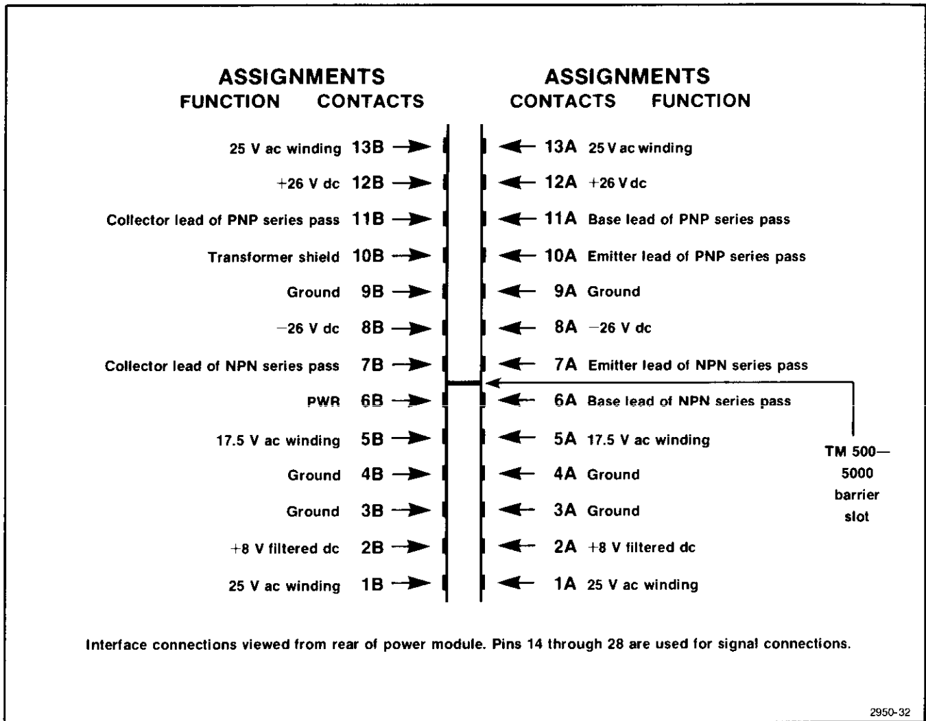
Fig. 5-13. Rear interface connector assignments.
