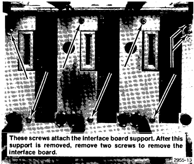
Fig. 5-6. Removal of interface circuit board.
