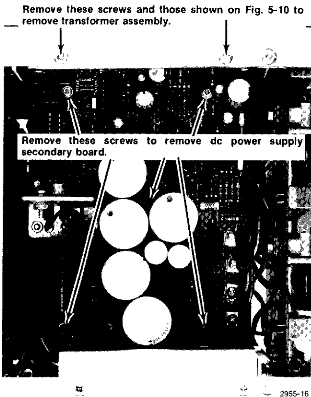
Fig. 5-9. Secondary board and partial primary transformer removal.
