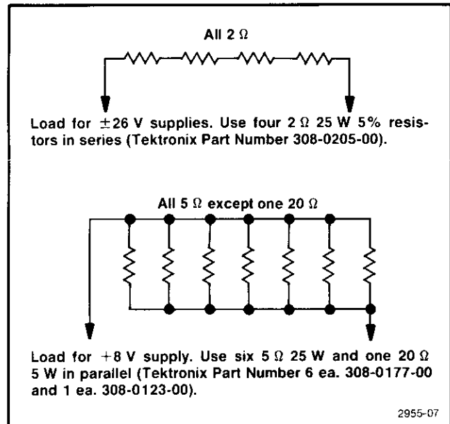
Fig. 4-1. Possible loads for use in performance check procedure. See text.
