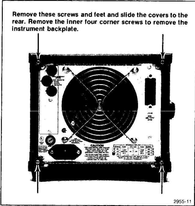
Fig. 5-4. Rear view of TM 5003.
